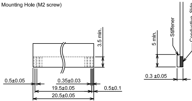
Recommended design rule for CN1 FPC
