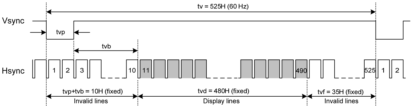
Fig. 9.2 Vertical Timing
