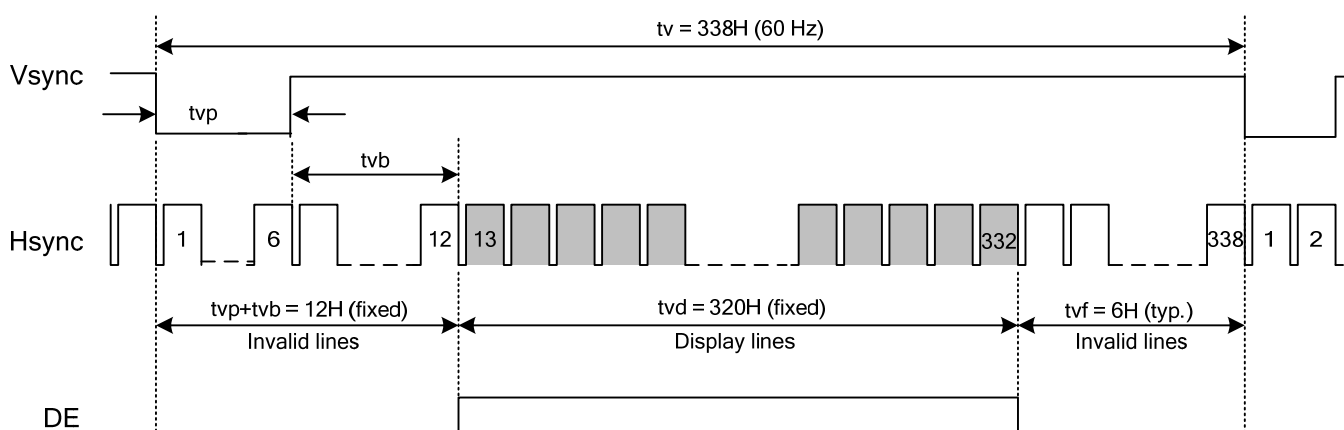
Fig. 9.2 Vertical Timing of Synchronous Mode
